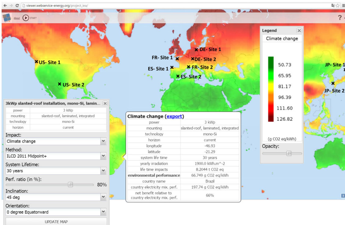
Figure 2. Worldwide map showing the evaluated sites and the climate change impacts for a 3-kWp mono-Si laminate integrated in a slanted roof with a 30-year lifetime, oriented to the south, with a 45° inclination in the “current” techno-economic context.
