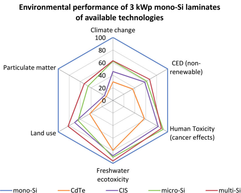
Figure 6. Radar chart for the comparative evaluation of the environmental performance of 3-kWp laminates of different technologies available in ENVI-PV: CdTe, CIS, micro-Si, mono-Si and multi-Si (results obtained for south orientation and 45° inclination) according to six environmental indicators from ILCD Midpoint+ method [20].
