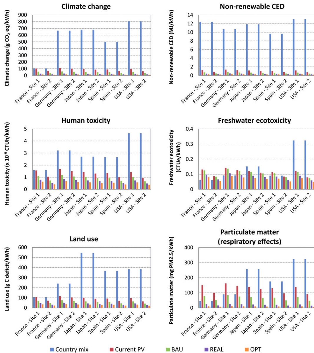
Figure 3. Environmental performances (impact/kWh of electricity generated) of "current" and "prospective" mono-Si systems (lifetimes according to Table II) for a 3-kWp mono-Si laminate integrated in a slanted roof; oriented to the south, with a 45° inclination compared to the current country electricity mix. Environmental indicators according to ILCD 2011 Midpoint+ method [20]: Climate change, Cumulative Energy Demand (CED, nonrenewable), Human toxicity (cancer effects), Freshwater ecotoxicity, Land use and Particulate matter (respiratory effects).
