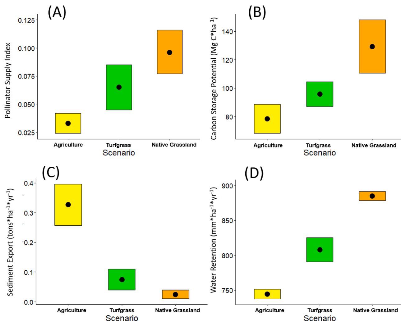
Fig. 3. Average ecosystem service values for the thirty Midwest solar facilities modeled with InVEST: (A) pollinator supply, (B) carbon storage, (C) sediment export, and (D) water retention. Tiles represent the upper- and lower-bound estimates based on the 25% and 75% quartiles. Points represent the midpoint average values.
