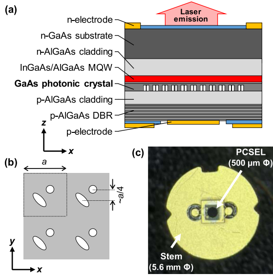
Fig. 2. (a) Cross-sectional schematic of a PCSEL. (b) Schematic structure of a double-lattice photonic-crystal. (c) External appearance of the 500- \mu\text{m} PCSEL packaged into a 5.6-mm- \varphi stem.
