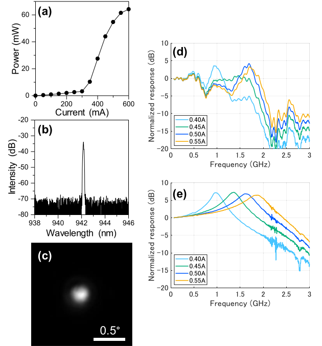
Fig. 3. Device characteristics of the 250- \mu\text{m} PCSEL: (a) I-L curve, (b) lasing spectrum at 520 mA, (c) far-field pattern at 500 mA, and (d) measured frequency response of the system, and (e) measured intrinsic frequency response of the PCSEL, which was obtained by subtracting the frequency response of the electrical system from the data shown in (d).
